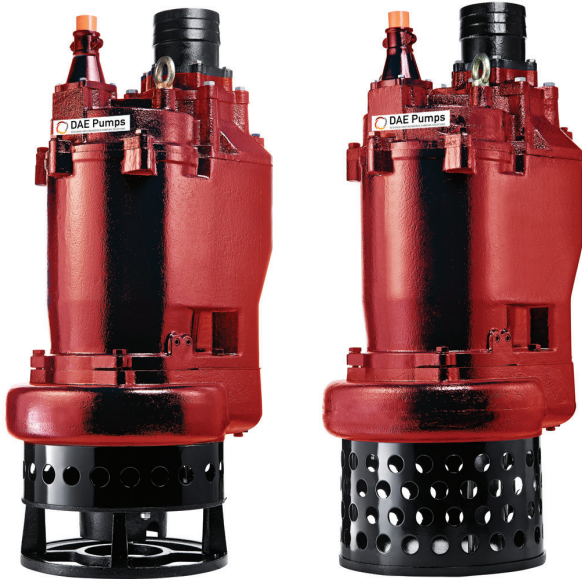
Opened Impeller
