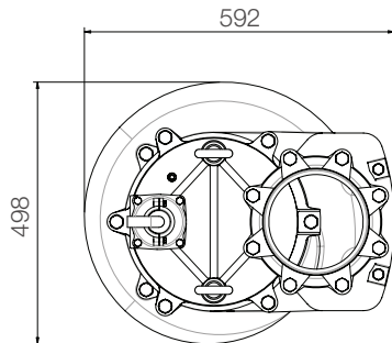
Opened Impeller
