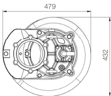
Opened Impeller
